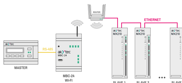
Master in RS-485 network - Slave in Wi-Fi network
