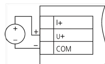
Voltage sensor wiring
