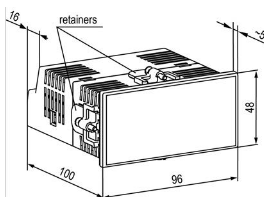
Dimensions of P2
