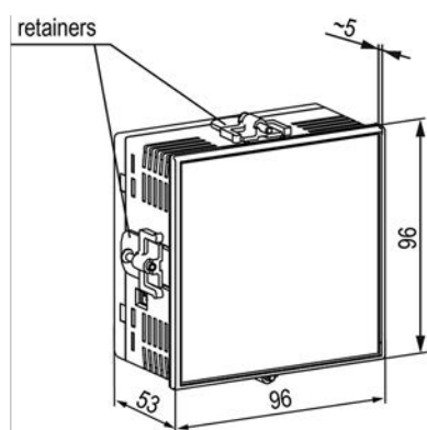
Dimensions of P1
