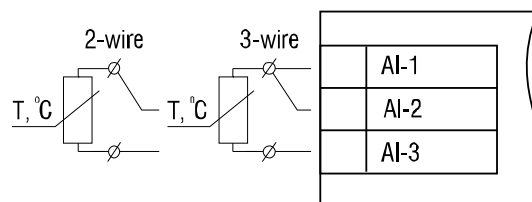
RTD sensor wiring
