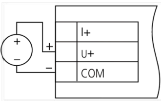
Voltage sensor wiring
