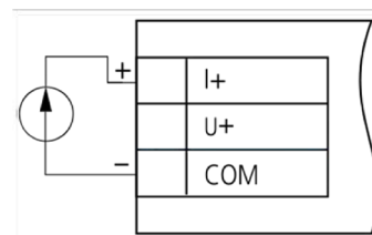
Current sensor wiring
