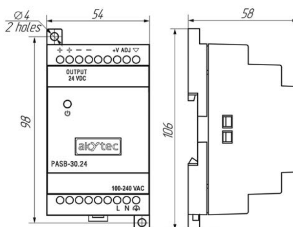
PASB-30.24
