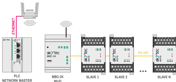
Master in Wi-Fi network - Slave in RS-485 network
