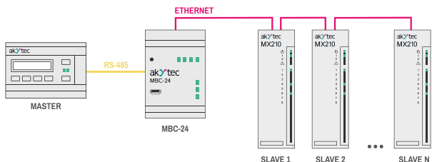
Master in RS-485 network - Slave in Ethernet network
