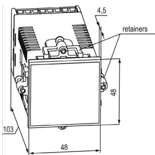
Dimensions of P5
