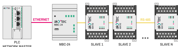
Master in Ethernet network - Slave in RS-485 network
