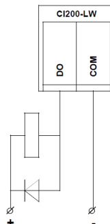
Fig. 8.3 External device connection diagram
