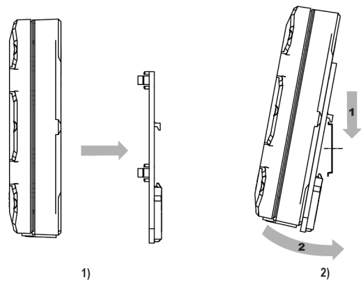
Abb. 9.1 DIN-Schiene montage
