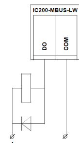
Fig. 3 – External device connection diagram
