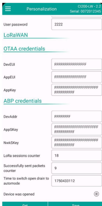
Fig. 11 – LoRaWAN settings
