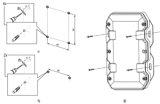
Fig. 9.2 Wall mounting
