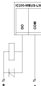
Fig. 8.3 External device connection diagram
