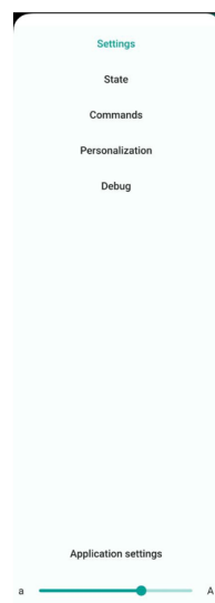
Fig. 5.3 Drop-down menu
