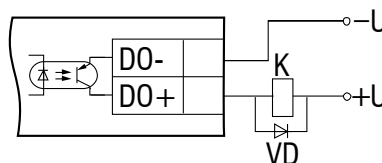
Fig. 5.7 Salida transistor NPN
