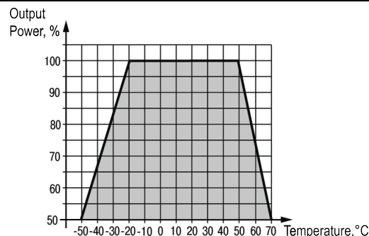
Fig. 1 – Output Power vs. Ambient Temperature
