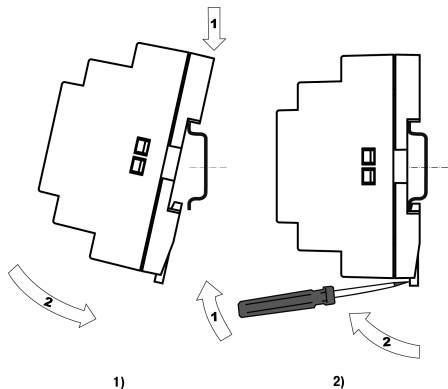
Fig. 6 – Installation (1) and Removing (2)
