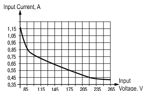
Fig. 3 – Input Power Supply Current vs. Input Power Supply Voltage
