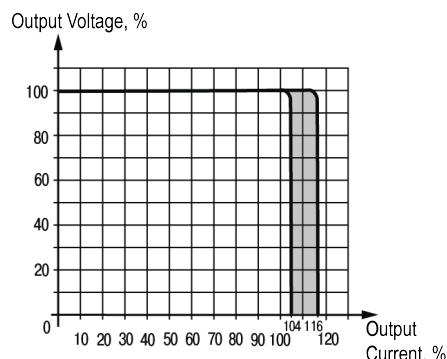
Fig. 2 – Output Voltage vs. Output Current
