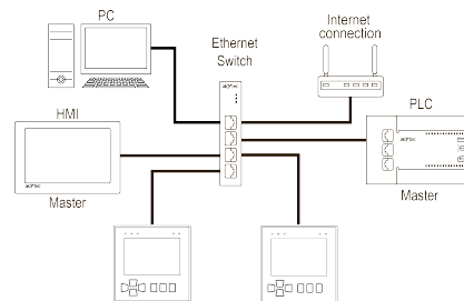
Fig. 12 – Star topology
