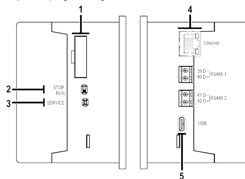
Fig. 16 – Side surfaces
