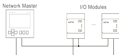
Fig. 14 – PR225 as Master
