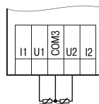
Fig. 5 – RTD sensors wiring
