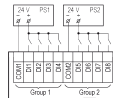
Fig. 4 – Switch contacts wiring
