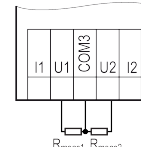
Fig. 6 – Resistance sensors wiring
