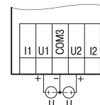
Fig. 8 – Voltage sensors wiring
