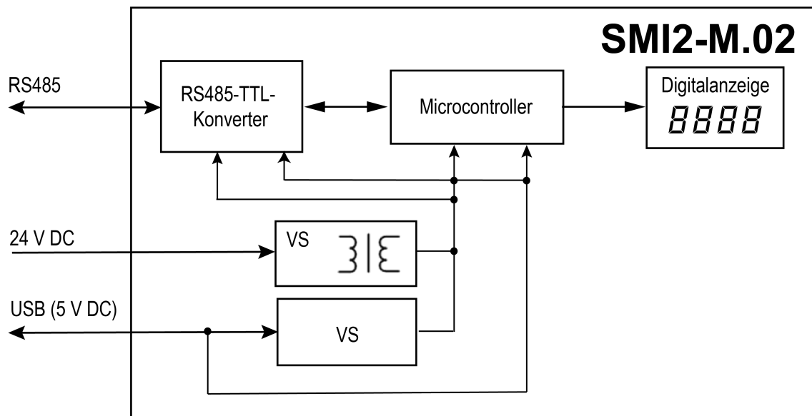
Abb. 2.2 Hardware-Blockdiagramm
